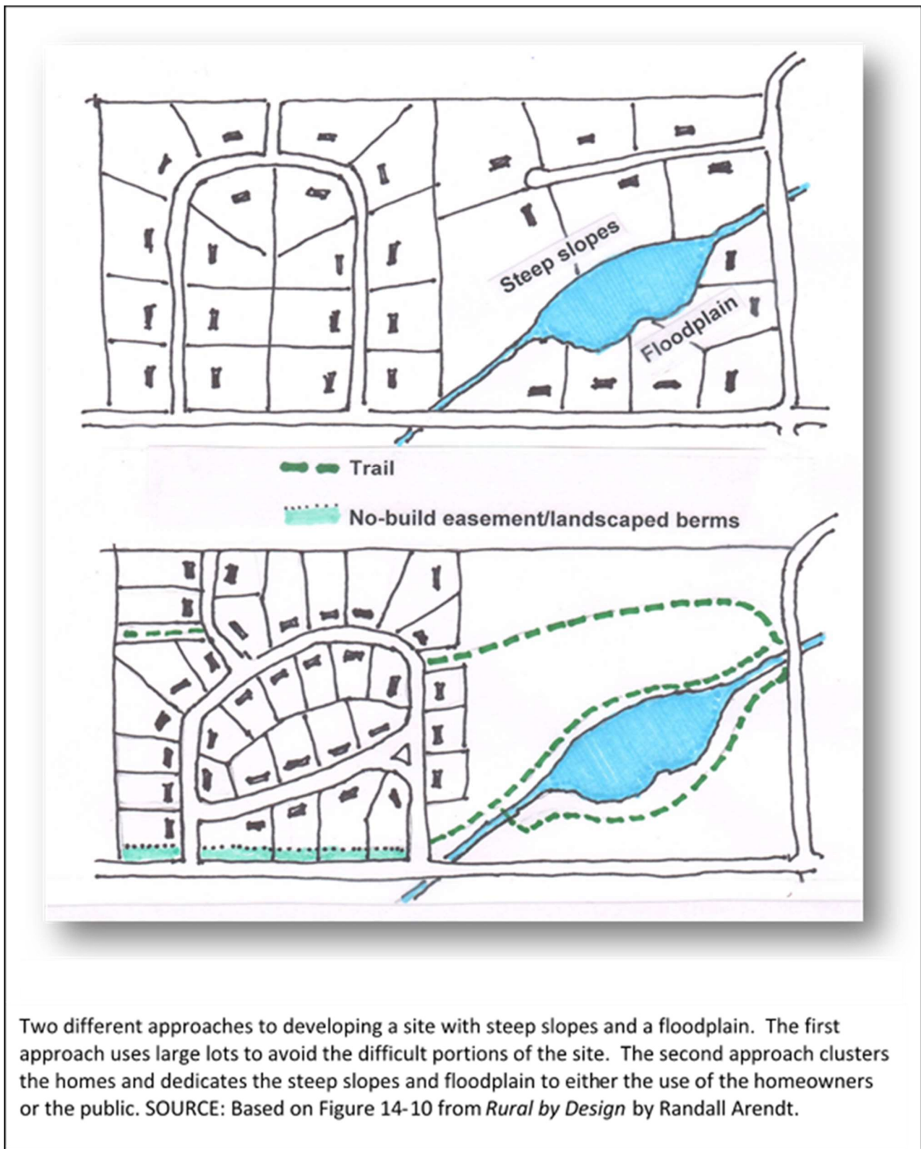
FIGURE 5. TWO DIFFERENT APPROACHES TO ADDRESSING STEEP SLOPES AND A FLOODPLAIN.
